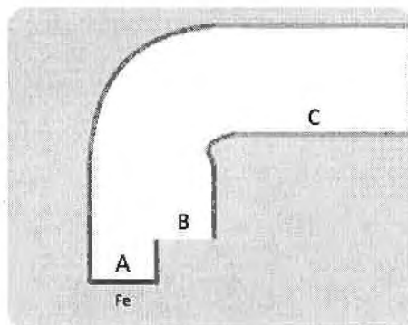
Figure 1 Stylized depiction of the CYP2E1 active site (A), cooperative site (B), and access channel (C).
