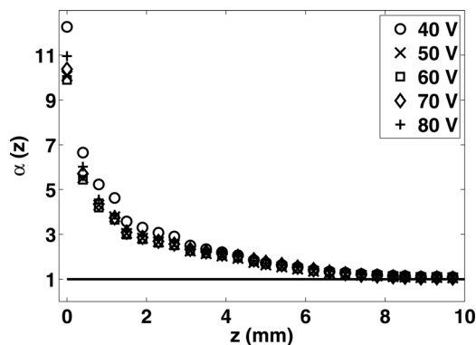
FIG. 4. The ratio of the ion density to the electron density, \alpha(z) , in the sheath for various driving potentials, V_{RF} , at 20 Pa obtained from the fluid model. The horizontal line indicates where the electron and ion densities are equal.
