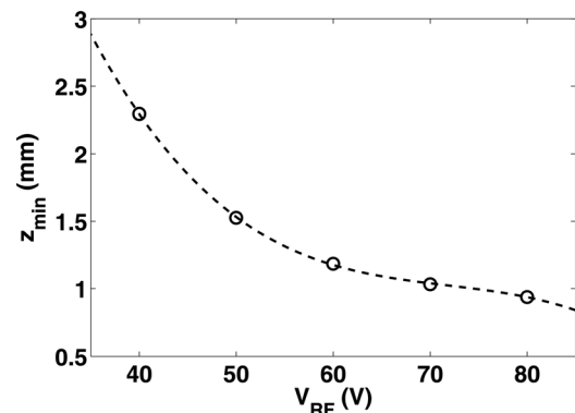
FIG. 10. The minimum levitation height for dust particles as a function of RF voltage as obtained in the fluid model. The dashed line is added to guide the eye.
